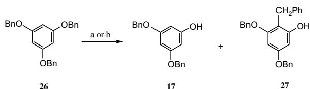
Scheme 4. Preparation of compound 27 : (a) EtSH/NaH/DMF, 150 °C; (b) BuSH/NaH/DMF, 150 °C.
