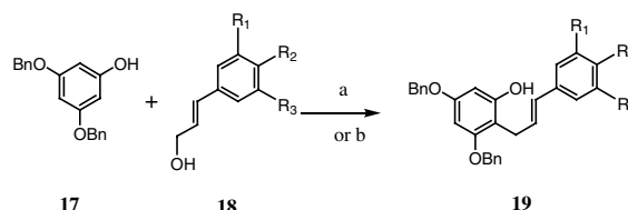
Scheme 1. Friedel–Crafts versus Mitsunobu condensation: (a) \text{H}_2\text{SO}_4/\text{SiO}_2/\text{CH}_2\text{Cl}_2 , rt; (b) \text{Ph}_3\text{P}/\text{DIAD}/\text{toluene} , -20^\circ\text{C} .
