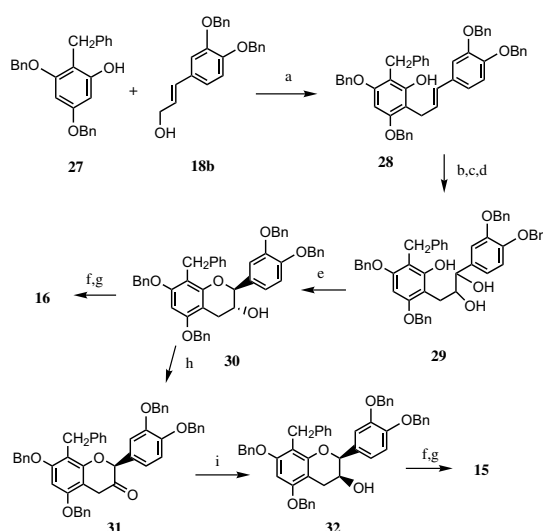
Scheme 5. Reagents and conditions: (a) H 2 SO 4 /SiO 2 /CH 2 Cl 2 , rt; (b) TBSCl/imidazole/DMF, rt; (c) AD-mix-β/MeSO 2 NH 2 /H 2 O/ t -BuOH/CH 2 Cl 2 /0 °C; (d) TBAF/THF, rt; (e) CH(OEt) 3 /PPTS/CH 2 Cl 2 , 60 °C; (f) 3,4,5-tris(benzyloxy)benzoyl chloride/DMAPI/CH 2 Cl 2 , rt; (g) H 2 /Pd(OH) 2 /MeOH/THF, rt; (h) Dess–Martin periodinane/CH 2 Cl 2 , rt; (i) L-Selectride/THF, –78 °C to rt.
