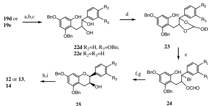
Scheme 3. Reagents and conditions: (a) TBSCl/imidazole/DMF, rt; (b) AD-mix- \alpha /MeSO 2 NH 2 /H 2 O/ t -BuOH/CH 2 Cl 2 /0 °C; (c) TBAF/THF, rt; (d) CH(OEt) 3 /PPTS/CH 2 Cl 2 , rt; (e) AcBr/CH 2 Cl 2 /0 °C; (f) K 2 CO 3 /acetone, rt; (g) K 2 CO 3 /MeOH; (h) 3,4,5-tris(benzyloxy)benzoyl chloride/DMAP/CH 2 Cl 2 , rt; (i) H 2 /Pd(OH) 2 /MeOH/THF, rt.
