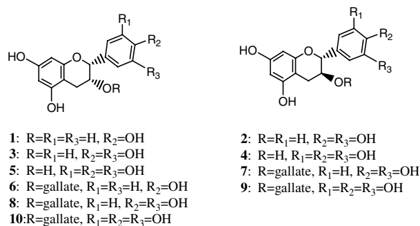
Figure 1. Various catechins in green tea.
