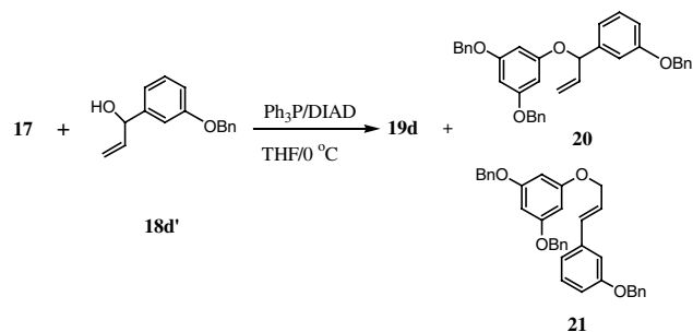
Scheme 2. Isolation of intermediate 20 .
