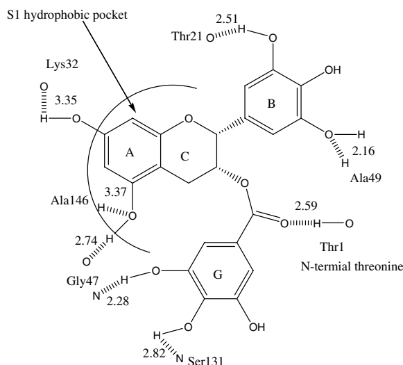
Figure 2. Docking model of (–)-EGCG in the \beta 5 -subunit of 20S proteasome. The number is distance in Å for the H-bond indicated.
